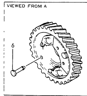
(7) CAMSHAFT
