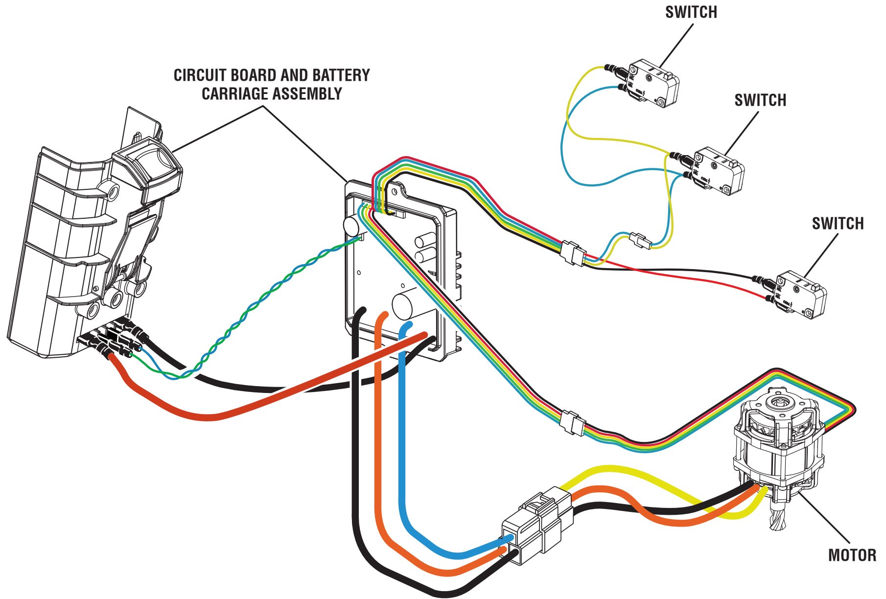
WIRING DIAGRAM
